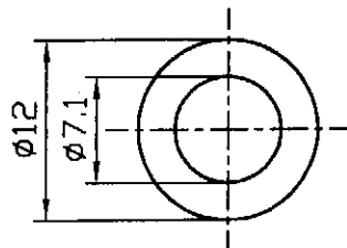
WASHER t=0.4
