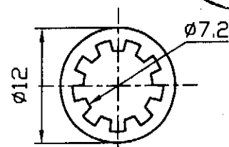
TEETH WASHER t=1.0
