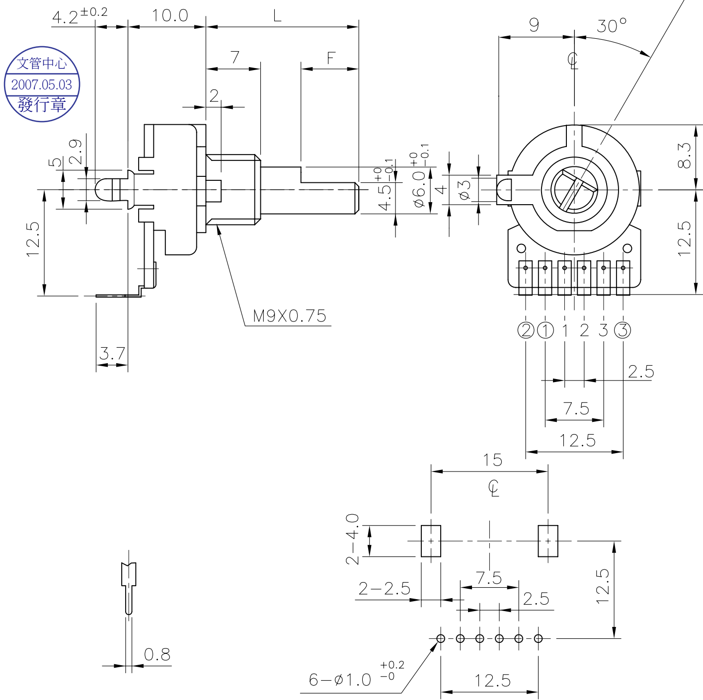
TERMINAL DETAIL
